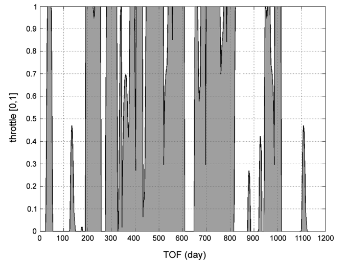
Fig. A1 Spacecraft's thrust history.
